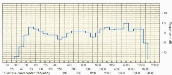
Frequency response of the 4311B taken with 1/3 -octave band pink noise. Measured at 1 m with a 1-watt input.
